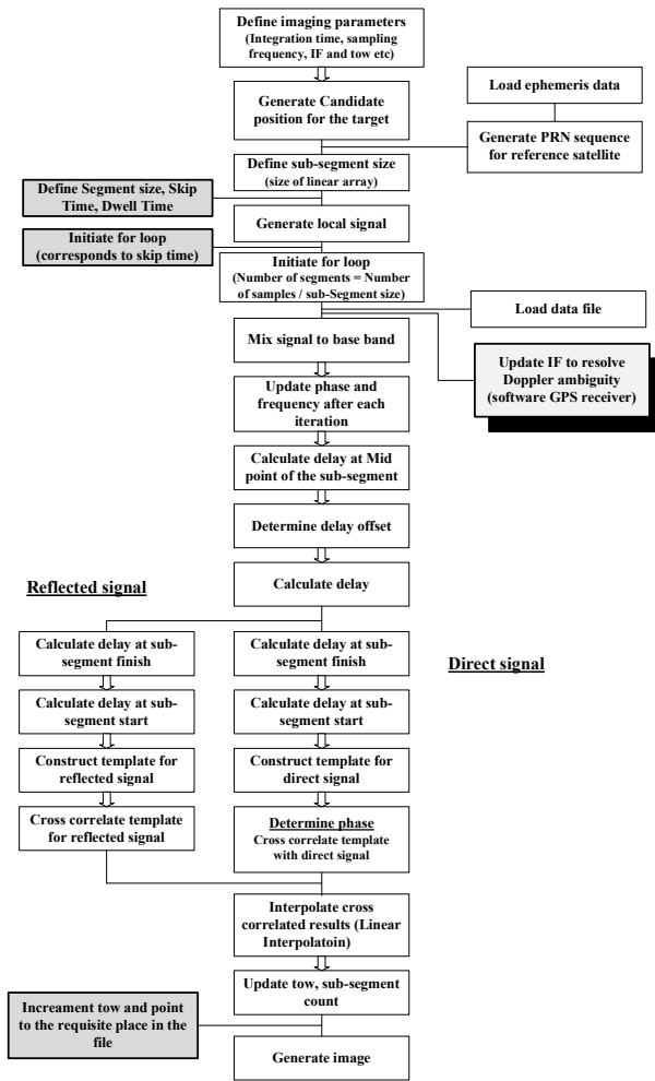
Figure 7: Block diagram of the reconstruction code
